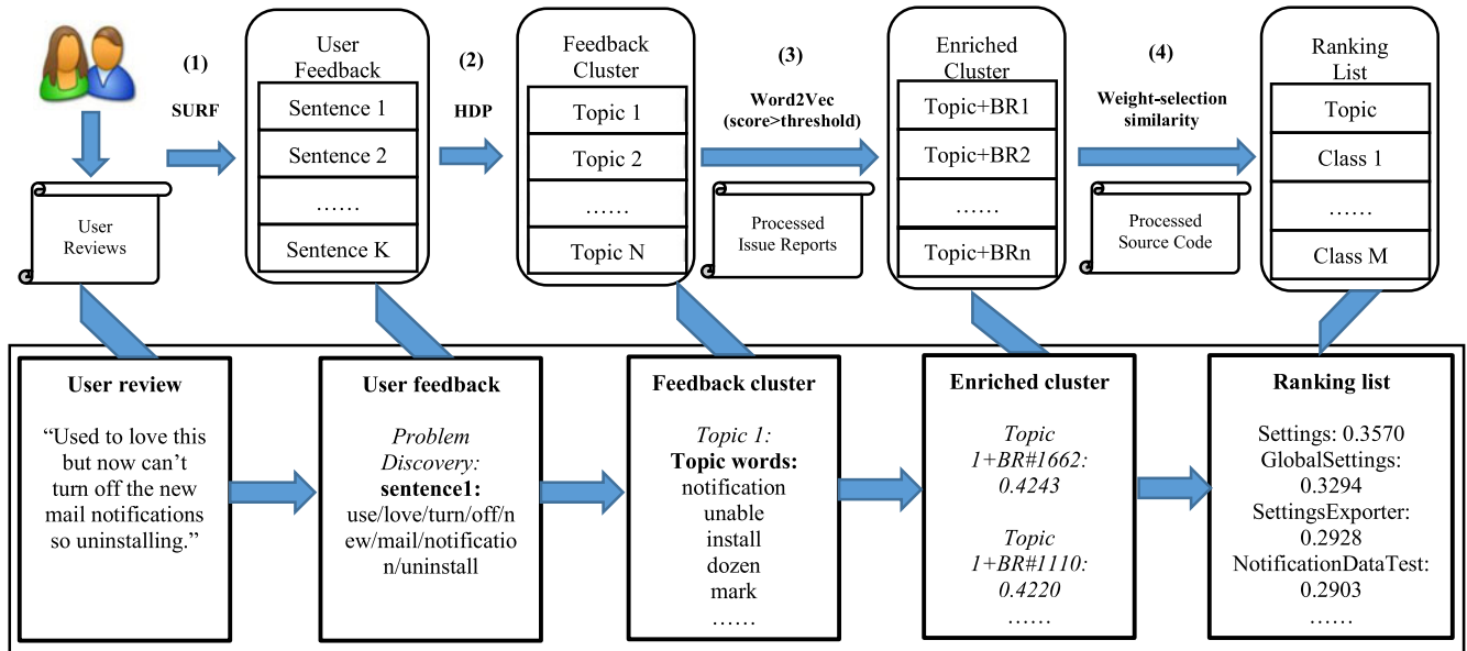
Fig. 4. Overall framework of Where2Change for user reviews in mobile apps.
