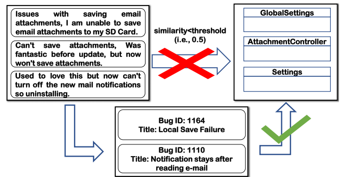
Fig. 3. Motivating example in K-9 Mail: change request localization.
