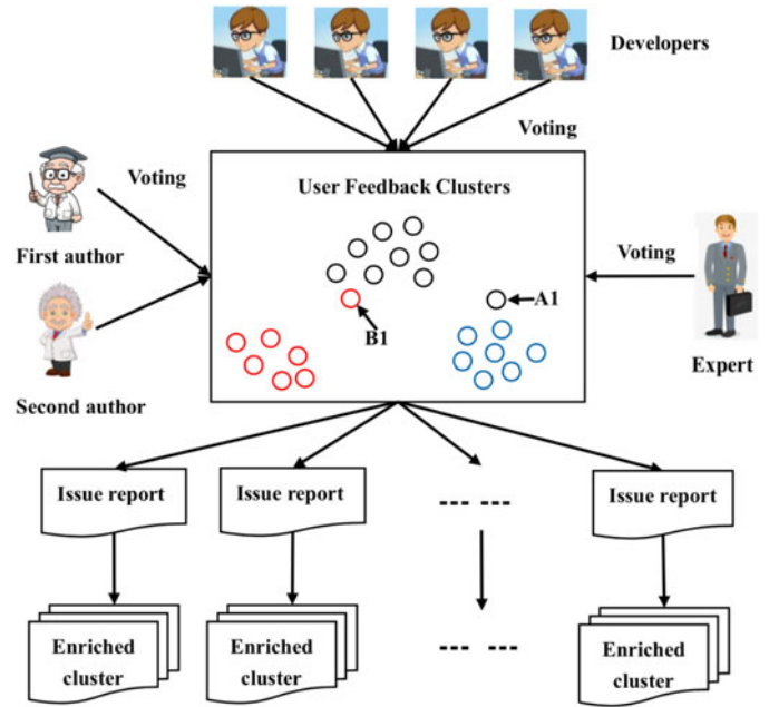
Fig. 5. Refinement process for the clustering results.
